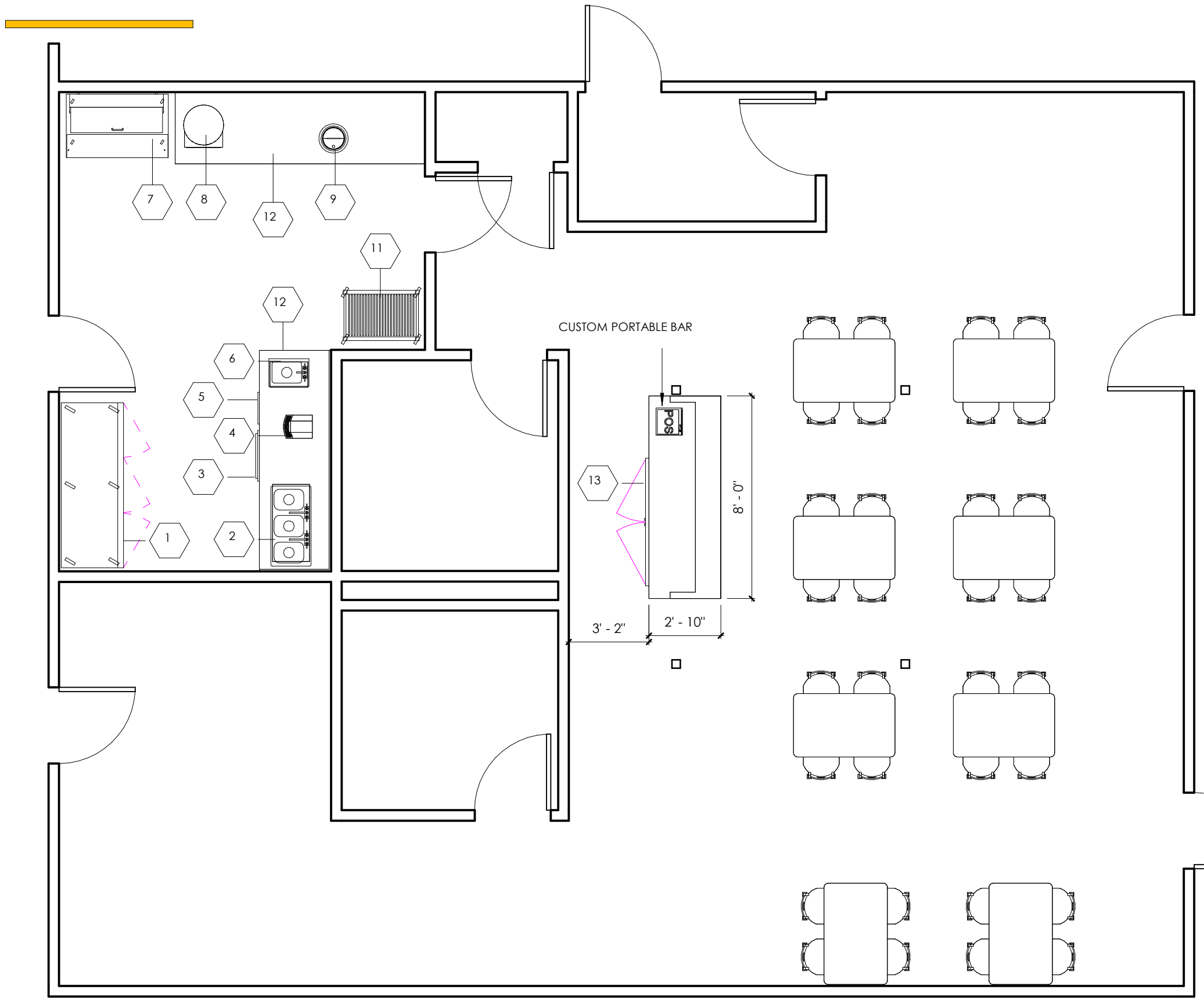
1 Floor Plan 1/4" = 1'-0"
