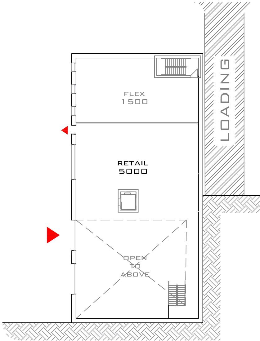
BASEMENT
