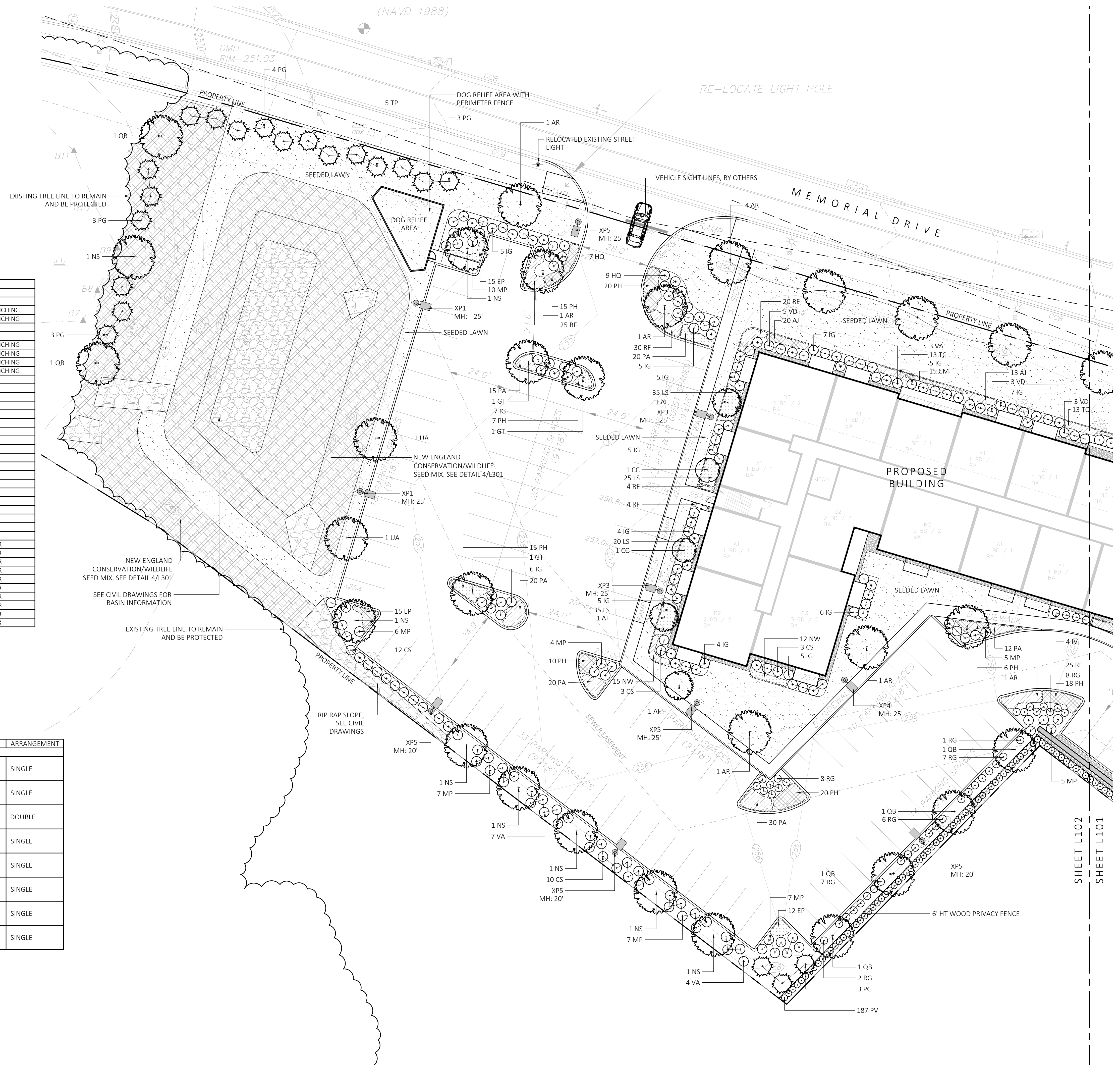
1 LANDSCAPE PLANTING AND LIGHTING ENLARGEMENT 1" = 10'-0"
