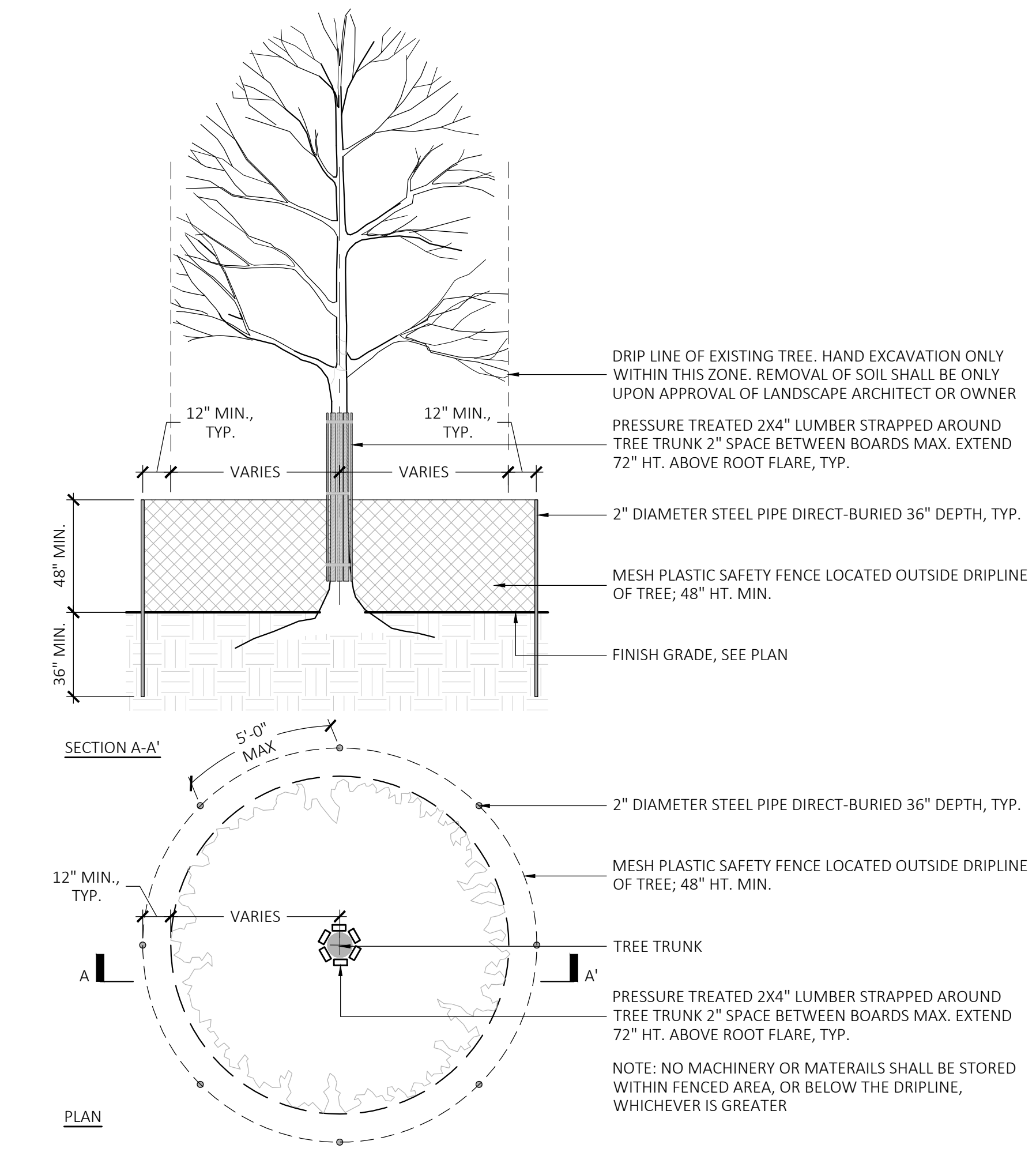
1 TREE PROTECTION SCALE: 1/4" = 1'-0"
