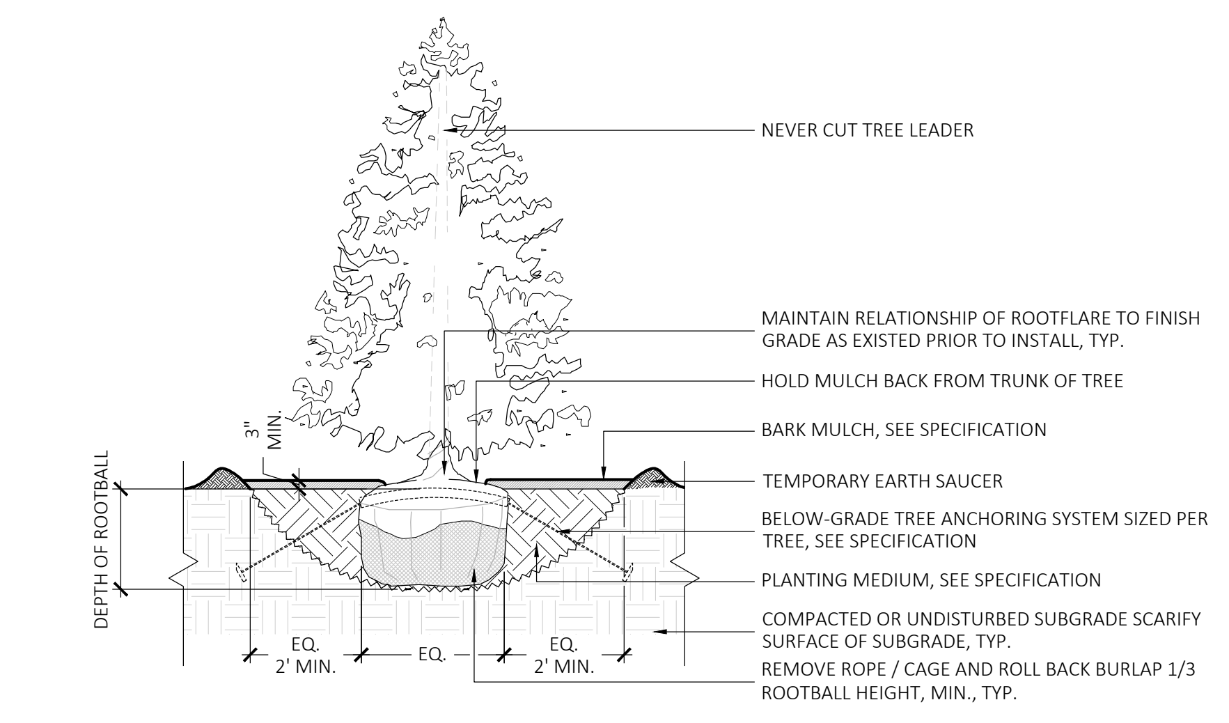
4 EVERGREEN TREE PLANTING SCALE: 1/4" = 1'-0"
