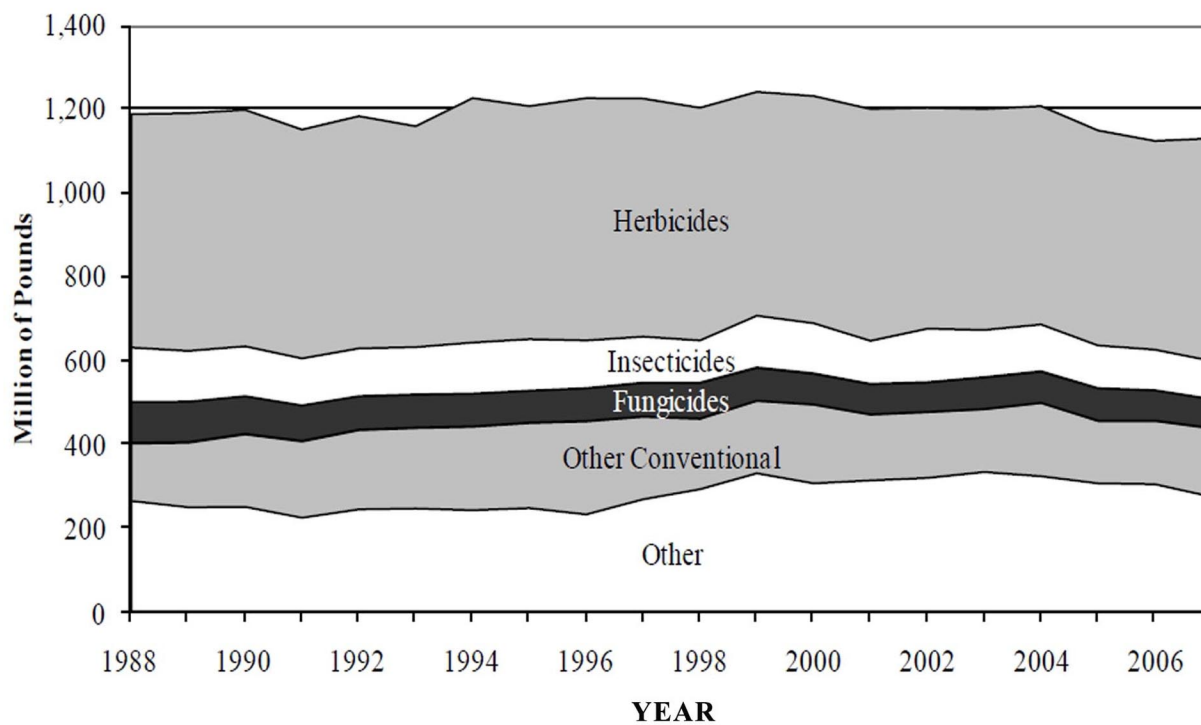
Annual Amount of Pesticide Active Ingredient Used in the United States by Pesticide Type, 1988–2007 Estimates All Market Sectors
