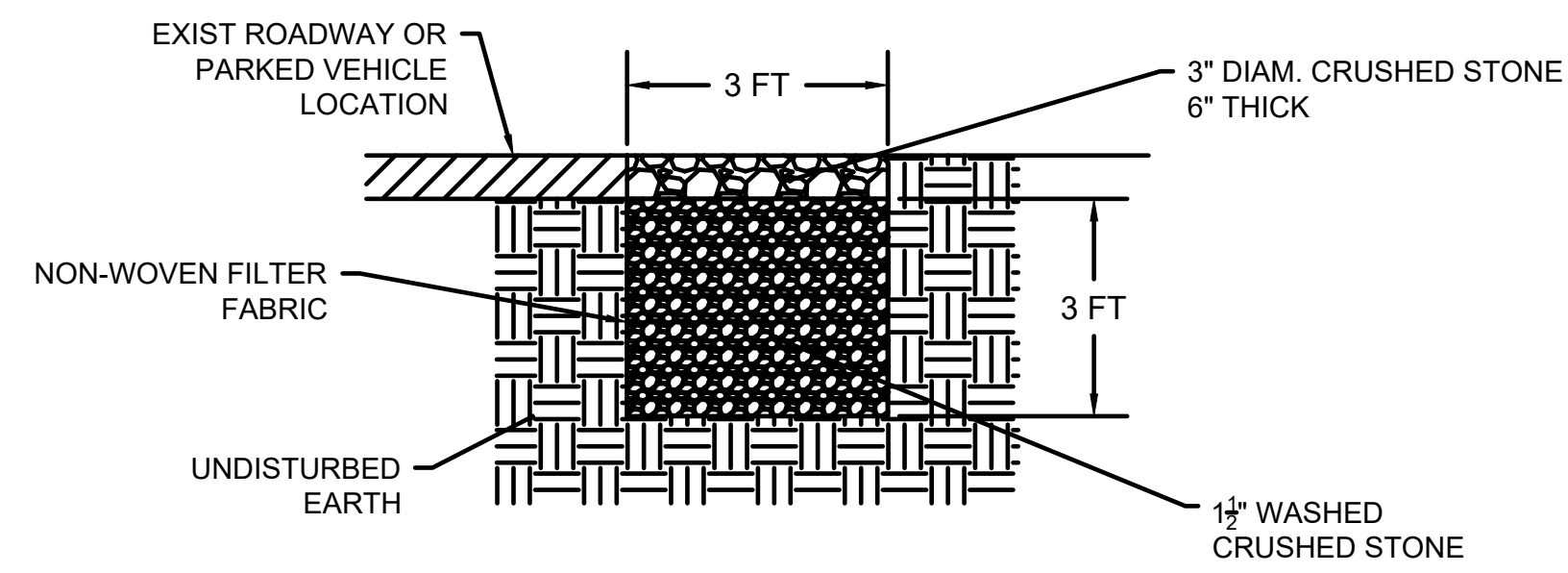
3-FT WIDE INFILTRATION TRENCH DETAIL N.T.S
