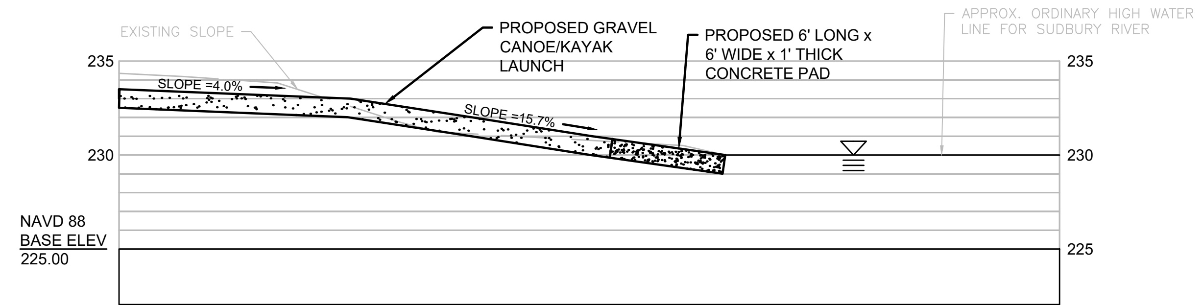
KAYAK/CANOE LAUNCH PROFILE SCALE: 1"=5'
